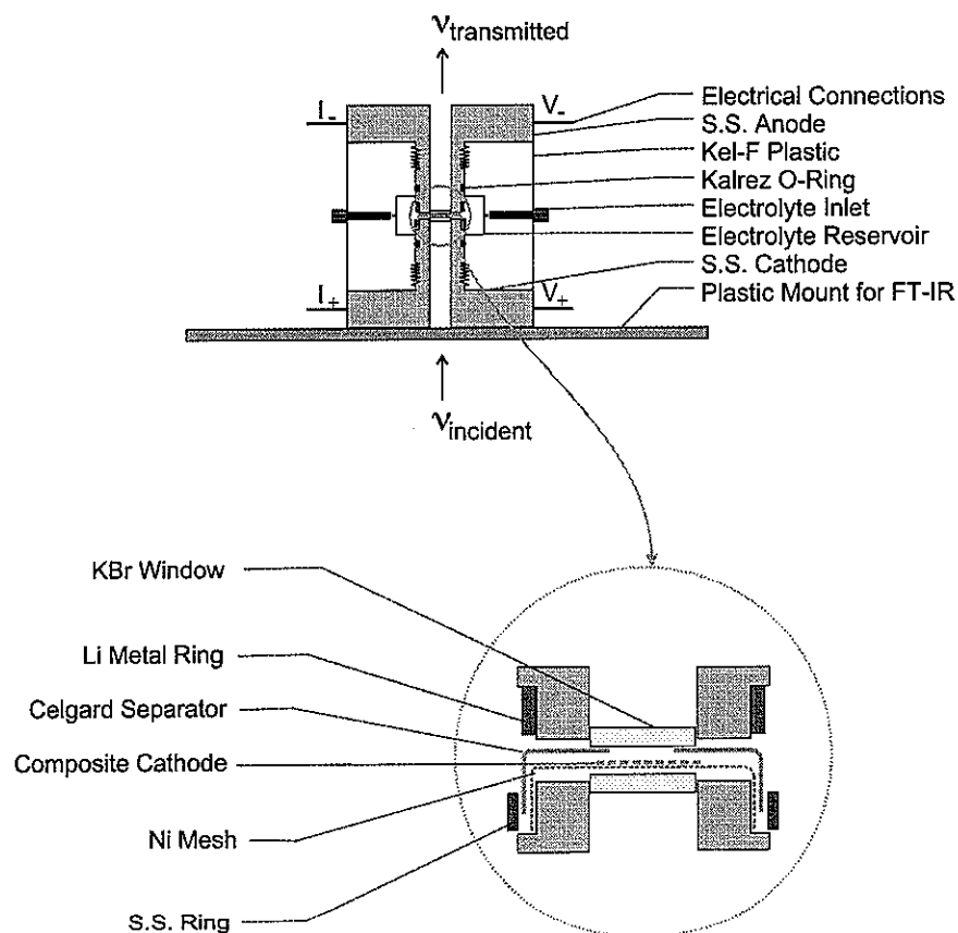
Figure 1. Schematic diagram of in situ IR transmission electrochemical cell.
