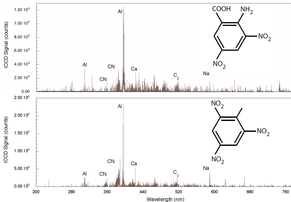
Figure 12: fs LIBS spectra of dinitroanthranilic acid (top) and of TNT (bottom) when each is deposited on an aluminum substrate.
