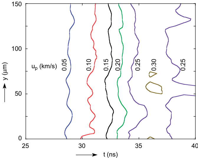
Fig. 24. Contours of constant free-surface velocity of shock front in y - t plane from simulation WHA-IV.
