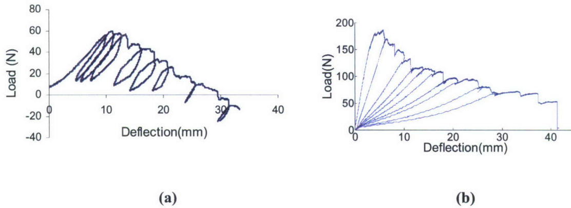
Figure 19. Load versus deflection plot from MCSB test of specimen with (a) 6 ply and (b) 12 ply face sheets.
