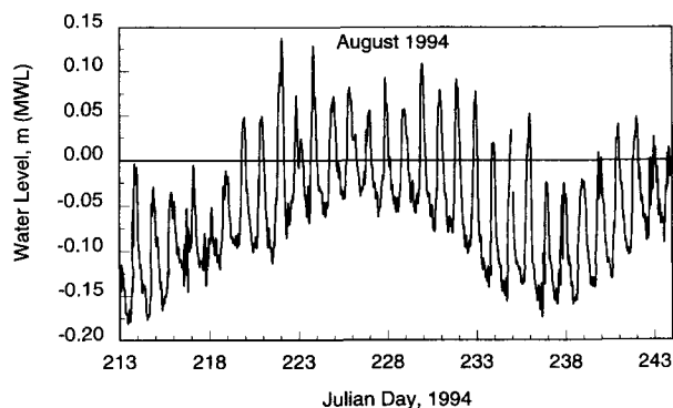
FIG. 7. Water level at Riviera, Texas, for Aug 1994.
