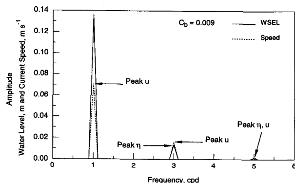
FIG. 2. Analytic solution: spectra of water-surface elevation and current, 1-m depth.
