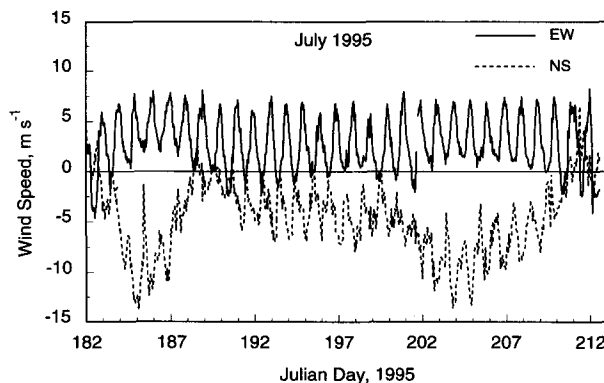
FIG. 9. Decomposed wind speed at Yarbrough, Texas, for Jul 1995.
