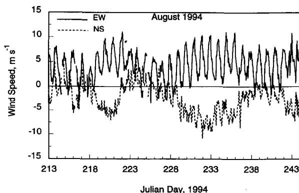
FIG. 5. Decomposed wind speed at Yarborough, Texas, for Aug 1994. North–south and east–west wind speeds are denoted by NS and EW, respectively. Positive values of the components indicate wind from the north and east.
