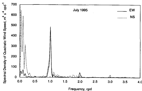
FIG. 10. Spectra of east–west and north–south components of quadratic wind speed measured at Yarbrough, Texas, Jul 1995.
