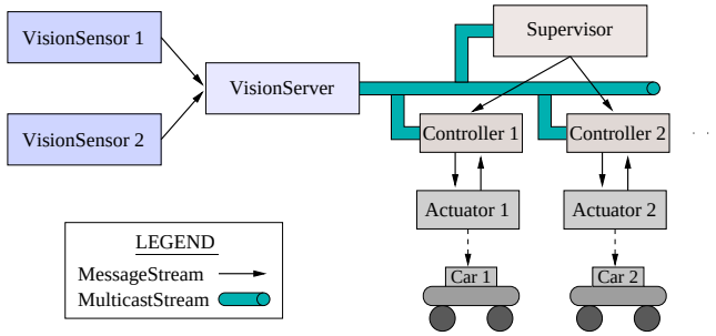
Fig. 7. Etherware based software architecture of the testbed
