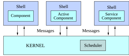
Fig. 5. Process architecture of Etherware
