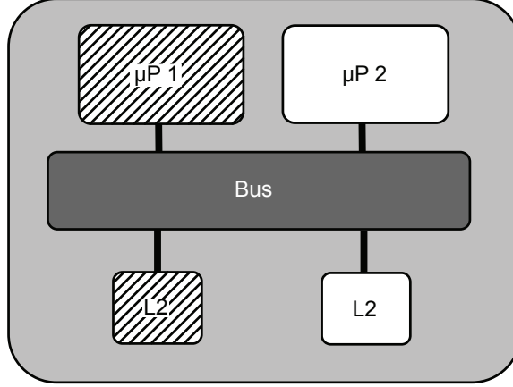
Figure 4: This figure shows a logical view of the computation plane after attaching the control plane. The control plane can prevent Processor 1 from accessing Processor 2 ’s portion of the L2 cache and vice-versa.
