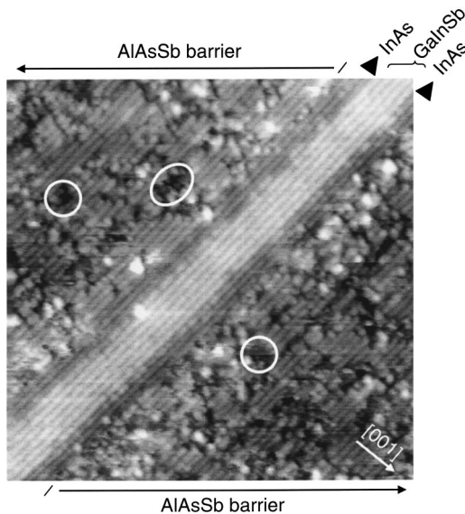
FIG. 3. Filled state XSTM image, 34 nm \times 34 nm, of an AlAsSb/InAs/GaInSb/InAs/AlAsSb active region grown at 435 °C. AlAs clusters are marked by white circles. The sample bias and tunneling current were -2.0 V and 0.07 nA, respectively.
