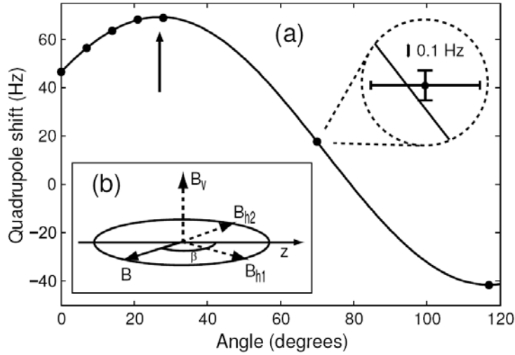
Figure 6: Dependence of the quadrupole shift \Delta on the orientation of the magnetic field with respect to the symmetry axis of the ion trap. The measurement is performed with a pair of ions in an entangled state. The atomic quadrupole moment is determined by measuring \Delta as a function of the electric field gradient that can be varied by changing the trap oscillation frequency.
