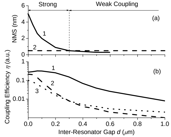
Fig. 2. (a) Normal mode splitting in resonant case as a function of d (line 1). (b) The coupling efficiency ( \eta ) as a function of d for different detuning ( \Delta ) between WGMs: 1 - \Delta=0.5 \text{ nm} , 2 - \Delta=5 \text{ nm} , 3 - \Delta=-7.5 \text{ nm} .
