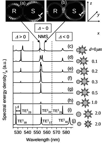
Fig. 1. (a) Antibonding and (b) bonding states. (c-h) Spectral energy density in receiving (R) sphere for different gaps ( d ). (i,j) spectra of WGM eigenstates.
