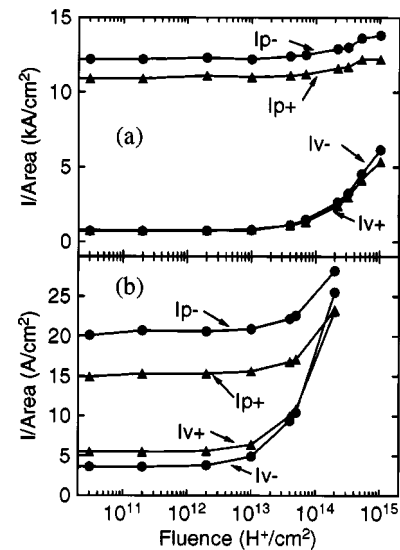
FIG. 2. Fluence dependence for the positive and negative bias peak currents, I_{p+} , I_{p-} , and the valley currents I_{v+} , I_{v-} for (a) 5 ML and (b) 13 ML AlSb barrier samples.
