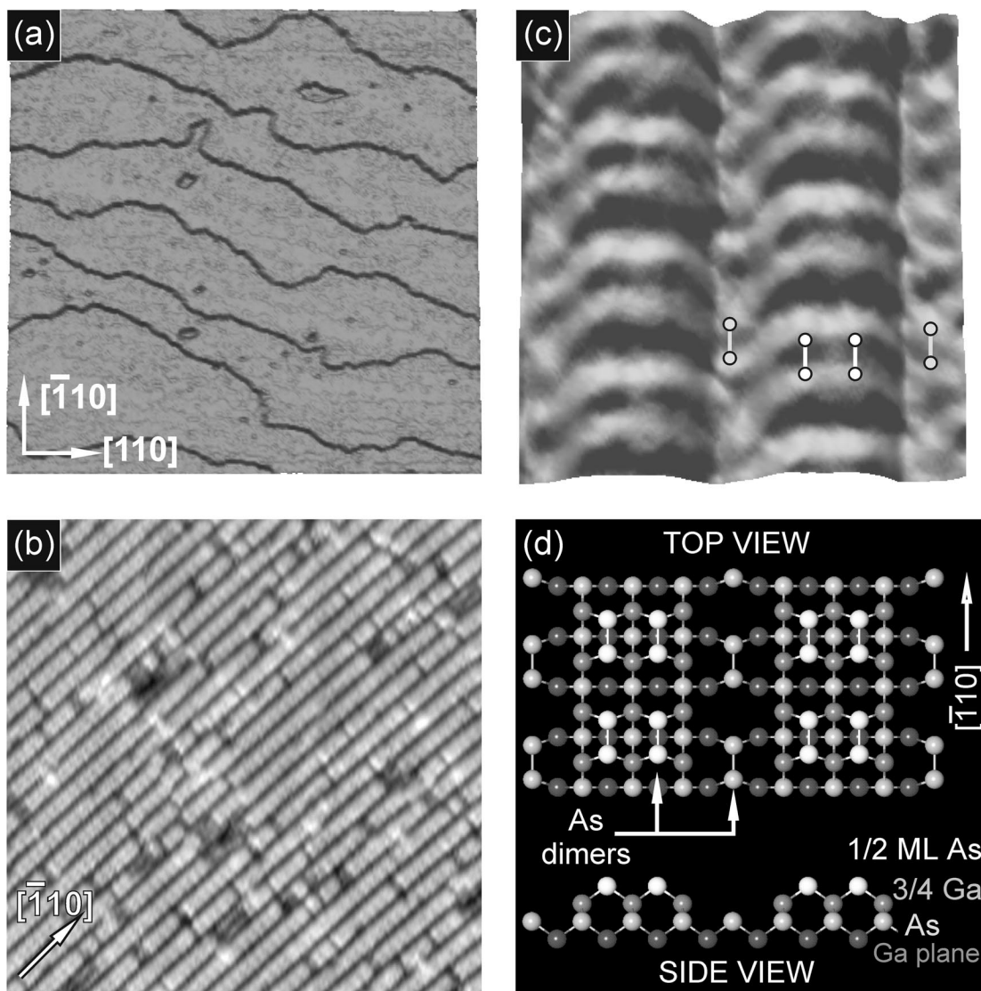
Fig. 1. (a) Large-area STM image (3D-rendered) showing the topography of an As-terminated GaAs(001)-(2×4) surface prepared by MBE with frequent growth interrupts (1.6 μm × 1.6 μm). (b) Higher magnification gray-scale image, 37 nm × 37 nm, showing the dimer rows of the reconstruction (filled states, 3.5 V, 30 pA). (c) 3.3 nm × 3.3 nm rendered view of the atomic-scale topography (filled states, 3.0 V, 0.1 nA). Note that the features associated with both the rows of As dimer pairs and the single row of As dimers in the layer below are just resolved. (d) A ball-and-stick model of the β 2 (2×4) reconstruction.
