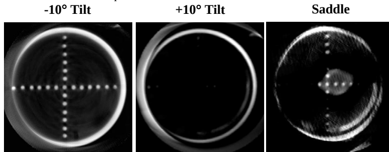
Figure 10: Reconstructed slice of the top spherical cross phantom acquired at (LEFT) -10°, (MIDDLE) +10° tilt, and (RIGHT) Saddle trajectory. As shown in the 3D CAD drawing, the top plane at the -10° tilt is more uniformly sampled. Even though more lesions are seen at the -10° tilt, 3D complex trajectories have less distortion and more complete sampling in the rest of the reconstruction volume.
