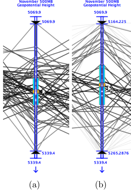
Fig. 5. A screen shot of the parallel coordinates application before (a) and after (b) scaling has been performed. In this example, scaling occurs by performing an upward mouse wheel function in the focus area of the axis which moves the values for the top and bottom closer together, effectively stretching the display upward and downward (with the base of the display fixed).
