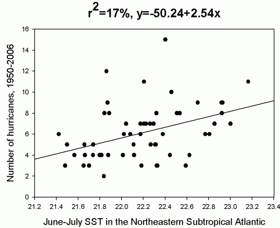
Fig. 1. A common visualization technique used in climate studies is the scatter plot overlaid with a linear regression line. This example shows the linear relationship between June–July SST in the northeastern subtropical Atlantic Ocean, and the number of hurricanes from 1950 to 2006. The explained variance is 17%.
