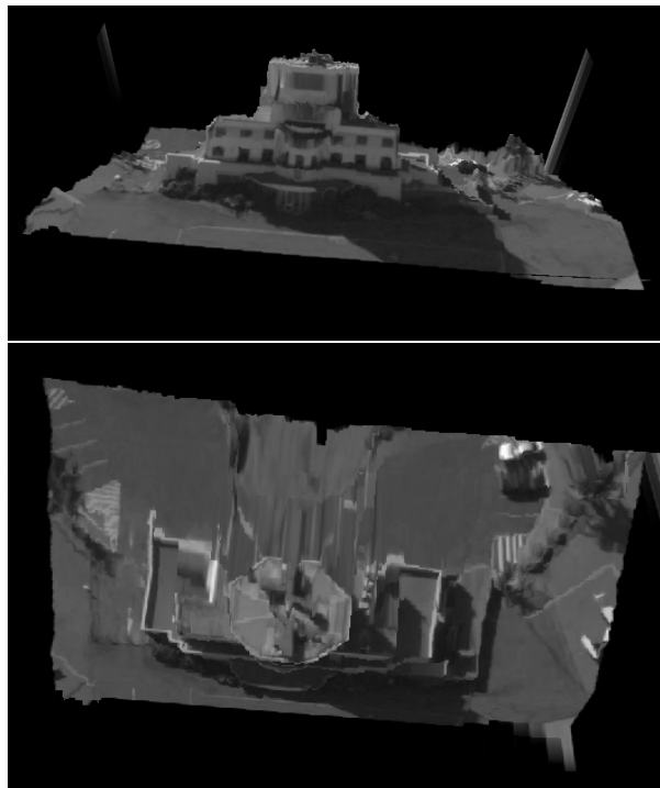
Figure 23: Two views of the VRML model produced using graph-cuts.
