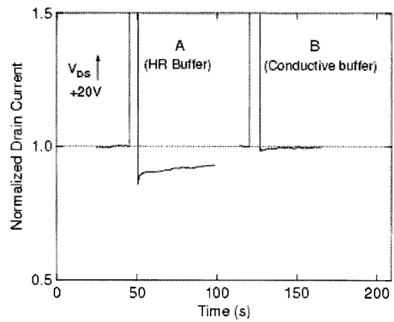
Fig. 5. Drain lag measurements. Drain current is normalized to the low-field value ( V_{DS} = 10 – 100 mV). “A”: Representative response for a device on a HR buffer. “B”: Device on a conductive buffer layer [6].
