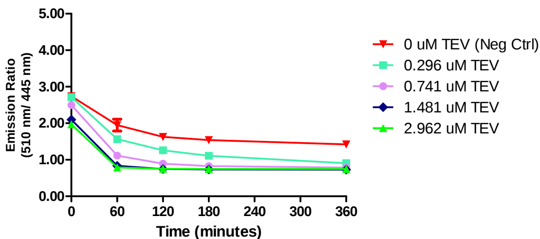
Figure : TEV Protease Cleavage of 1.38 \mu\text{M} FRET Protein in IVTT System
