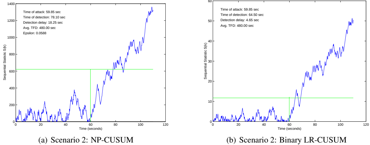
Figure 16: NP-CUSUM and B-CUSUM detection statistics
