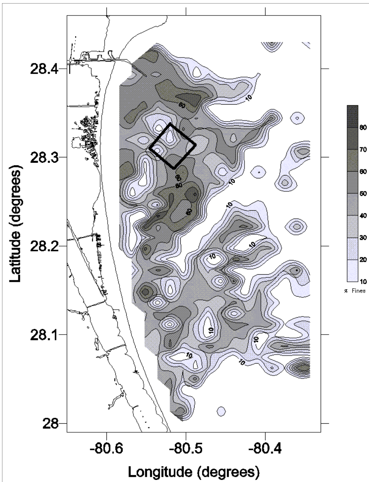
Figure 6: Gridded data (percent fines)
