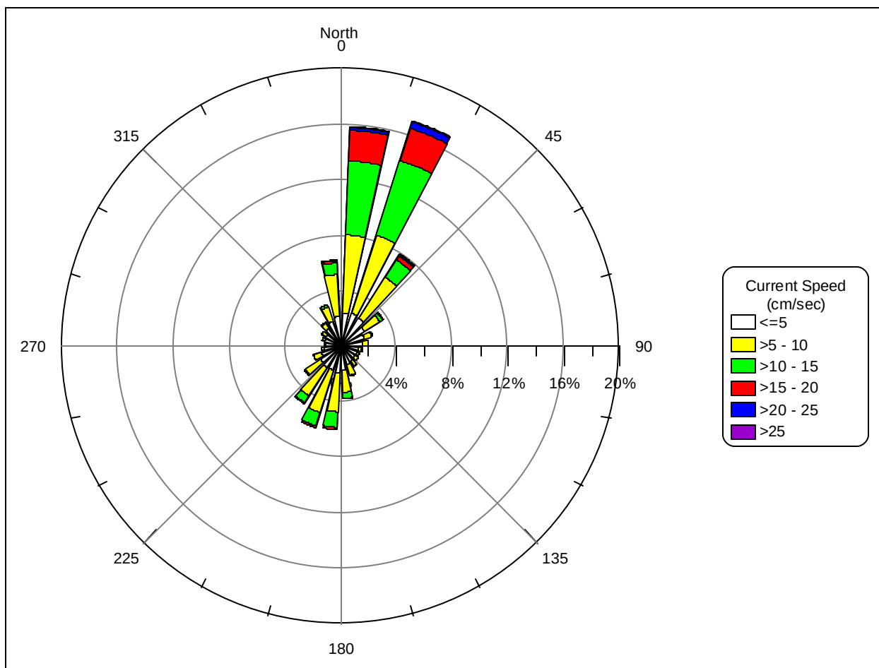
Figure 11: Depth Average Current Rose at the Canaveral ODMDS (EPA, 2004).
