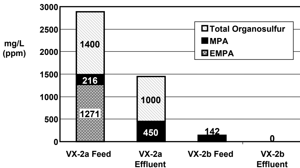
Figure 1. Degradation of CWC compounds by Method #1.
