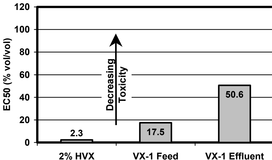
Figure 4. Microtox ® results with feed and effluents from Method #2.
