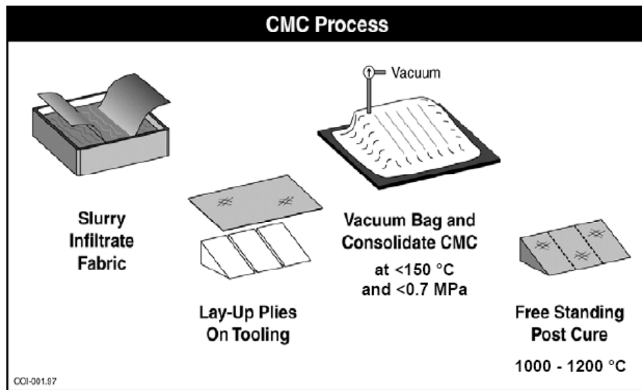
Figure 8. N720A manufacturing process. (Jurf)
