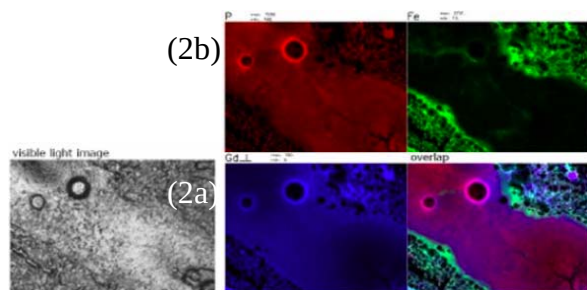
Figure 2. (a) Light micrograph of duct distended with DCIS. (b) Elemental concentration maps of P (red), Fe (green), Gd (blue) and the overlap demonstrating Gd (but not Fe) penetrated the mammary duct distended with DCIS.
