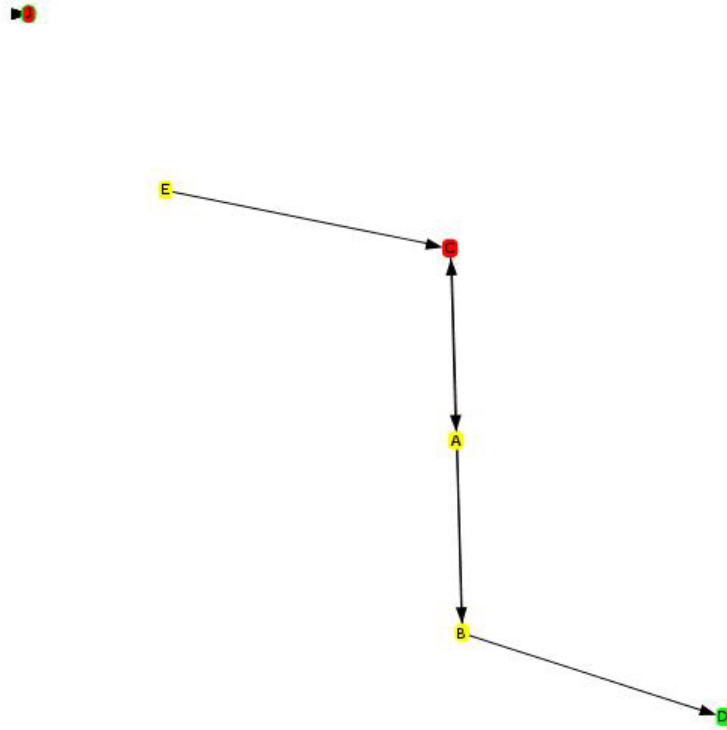
Figure 4.12: This diagram depicts the resultant radial visualization of dataset 4 in a radial display. Actor J was selected as the focus, then actor C was selected as both represent failed actors. This display has moved actor C over actor J, resulting in a misleading visualization.
