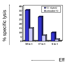
Figure 4: Cytotoxic activity of CTL by 51Cr-release assay
