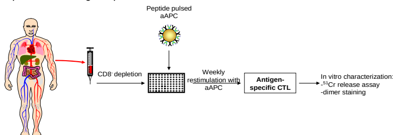
Figure 2 : Schematic for aAPC based induction and expansion of antigen-specific CTL
