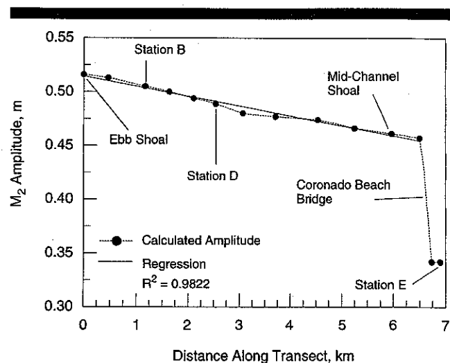
Figure 12. Calculated tidal amplitude at points ranging from the Atlantic Ocean (ebb shoal) to Station E (south of Coronado Beach Bridge).
