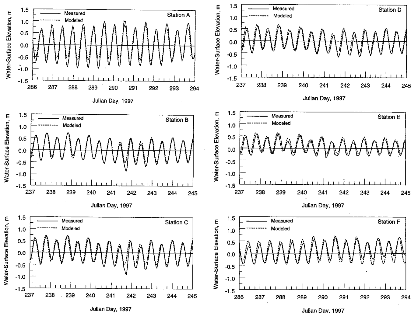
Figure 6. Representative measured and calculated water level (MSL) at instrument locations.
