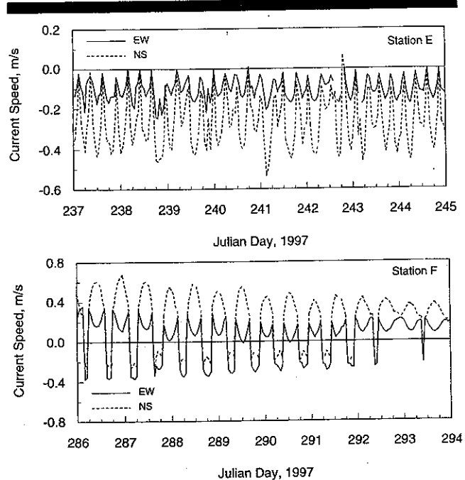
Figure 8. Representative measured current at Stations E and F. EW and NS denote flow parallel to the east-west and north-south axes, respectively. Positive values indicate flow toward the east and north.
