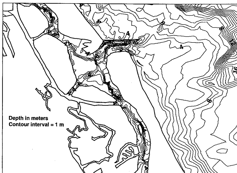
Figure 5. Bottom topography for the study area, relative to MSL.
