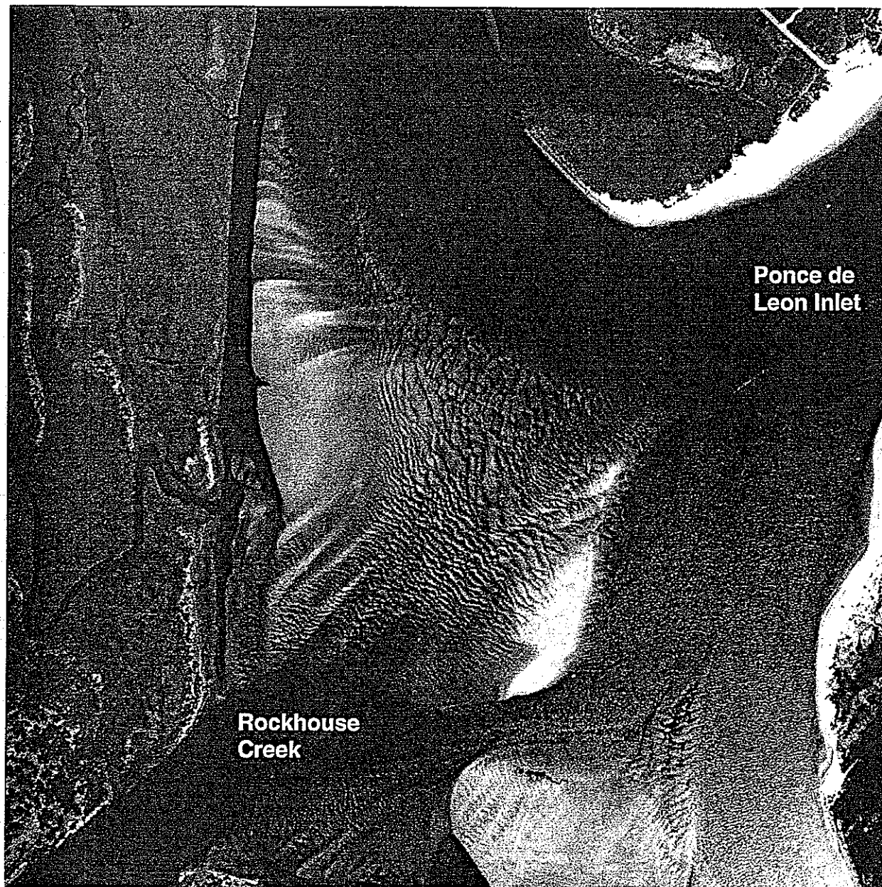
Figure 2. Aerial photograph taken March 21, 1996, showing the flood shoal west of Ponce de Leon Inlet. Rockhouse Creek splits the shoal into two lobes.
