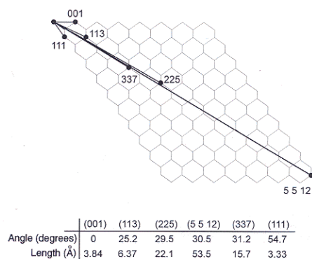
Fig. 1. Side view of a Si crystal lattice bounded by the (001) and (111) planes. The intersections of the lattice lines represent projections of atomic positions onto the {110} plane (the plane of the page). Six plane orientations on this lattice are indicated by line segments, with the length of each line equaling one unit cell of the associated bulk-terminated surface. The crystal truncation of one unit cell of (5 5 12) is equivalent to that of two unit cells of (337) plus one of (225). The table lists the angle with respect to the (001) plane and the bulk-terminated unit cell length for each orientation.
