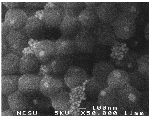
Figure 4. Scanning electron micrograph showing cluster of aggregated gold nanoparticles trapped in the interstices between latex particles in the bottom portion of droplet cap.
