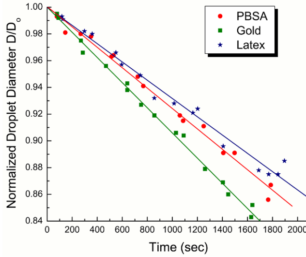
Figure 9. Droplet diameter variation with evaporation time for droplets containing different ingredients.
