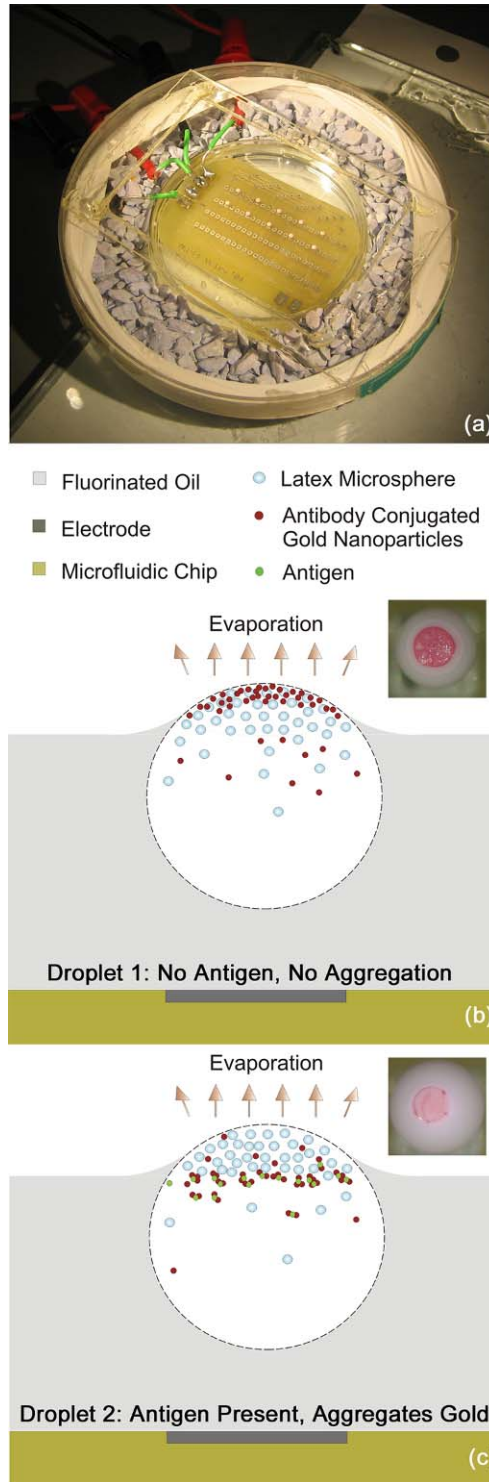
Figure 1. (a) Experimental setup with evaporating droplets on a DEP chip. (b) Schematics and optical micrograph from above of evaporating droplet without antigen. (c) Schematics and micrograph of gold nanoparticle aggregation in a droplet containing antigen.
