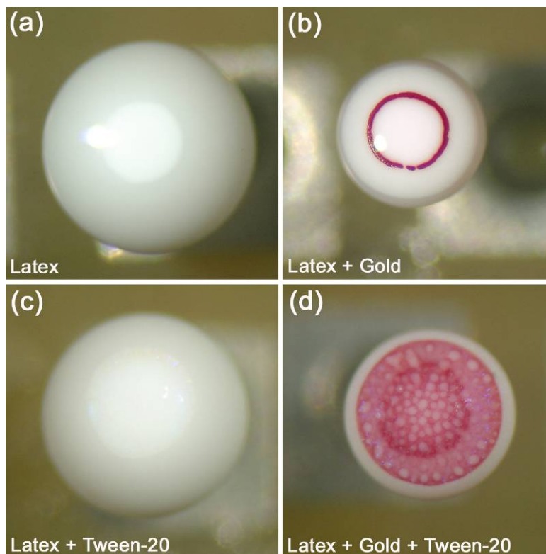
Figure 8. Micrographs of typical droplets, illustrating the effect of presence of gold nanoparticles and Tween-20 on the drying rate of droplets. (a) Latex only, (b) Latex and gold nanoparticles, (c) Latex and Tween-20, (d) Latex, gold nanoparticles and Tween-20. All droplets were allowed to evaporate for 65 minutes.
