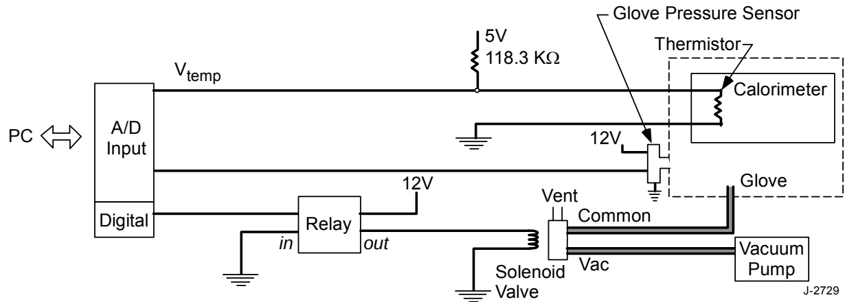
Figure 5. Schematic of control and signal acquisition.
