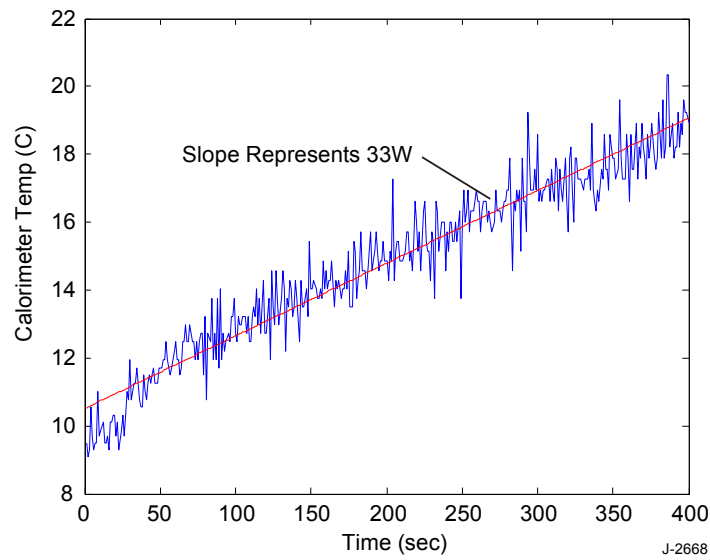
Figure 6. Typical calorimeter temperature record.
