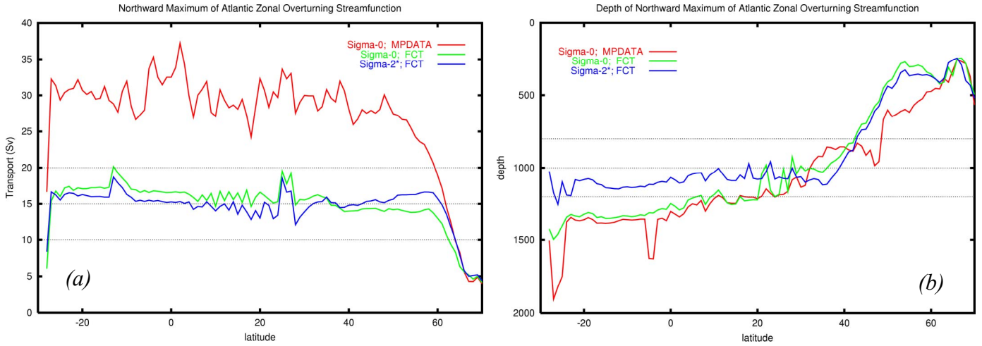
Figure 1. (a) Zonally-averaged northward transport (Sv) of the meridional overturning cell (MOC) vs. latitude, transport occurring above (b) the depth of the switch from net northward flow in the upper ocean to net southward flow below in the .08° Atlantic HYCOM using \sigma_0 coordinates with MPDATA (red) and FCT (green), and \sigma_2^* coordinates with FCT (blue). The MOC amplitude is too strong in the simulation with MPDATA, but in excellent agreement with observations in simulations with FCT advection. The switch from northward (upper) to southward (deep) flow is too deep in both the MPDATA and FCT \sigma_0 simulations, but much more realistic in the \sigma_2^* FCT simulation.
