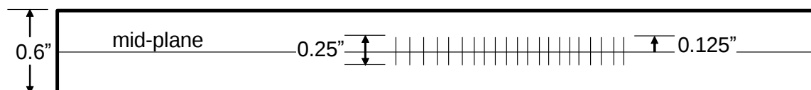
Figure 18: Schematic of Co-cured Z-pinned Baseline Specimen
