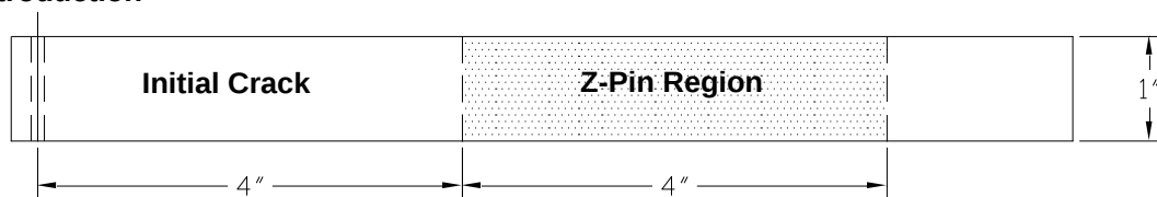
Figure 17: Schematic of Double Cantilever Beam Specimen
