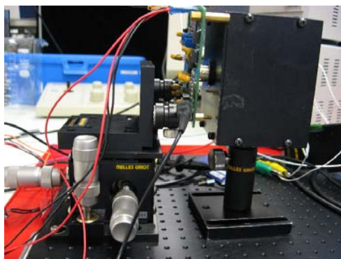
Figure 4-9: Integrating sphere 2500INT-2-IGAC and Keithley Model 2500 Dual Photodiode Meter for average power measurement
