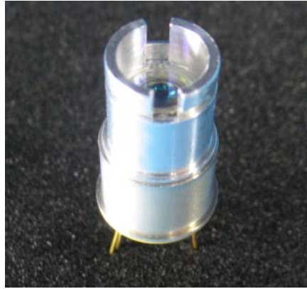
Figure 3-23: Completed TOSA with DP04 lens
