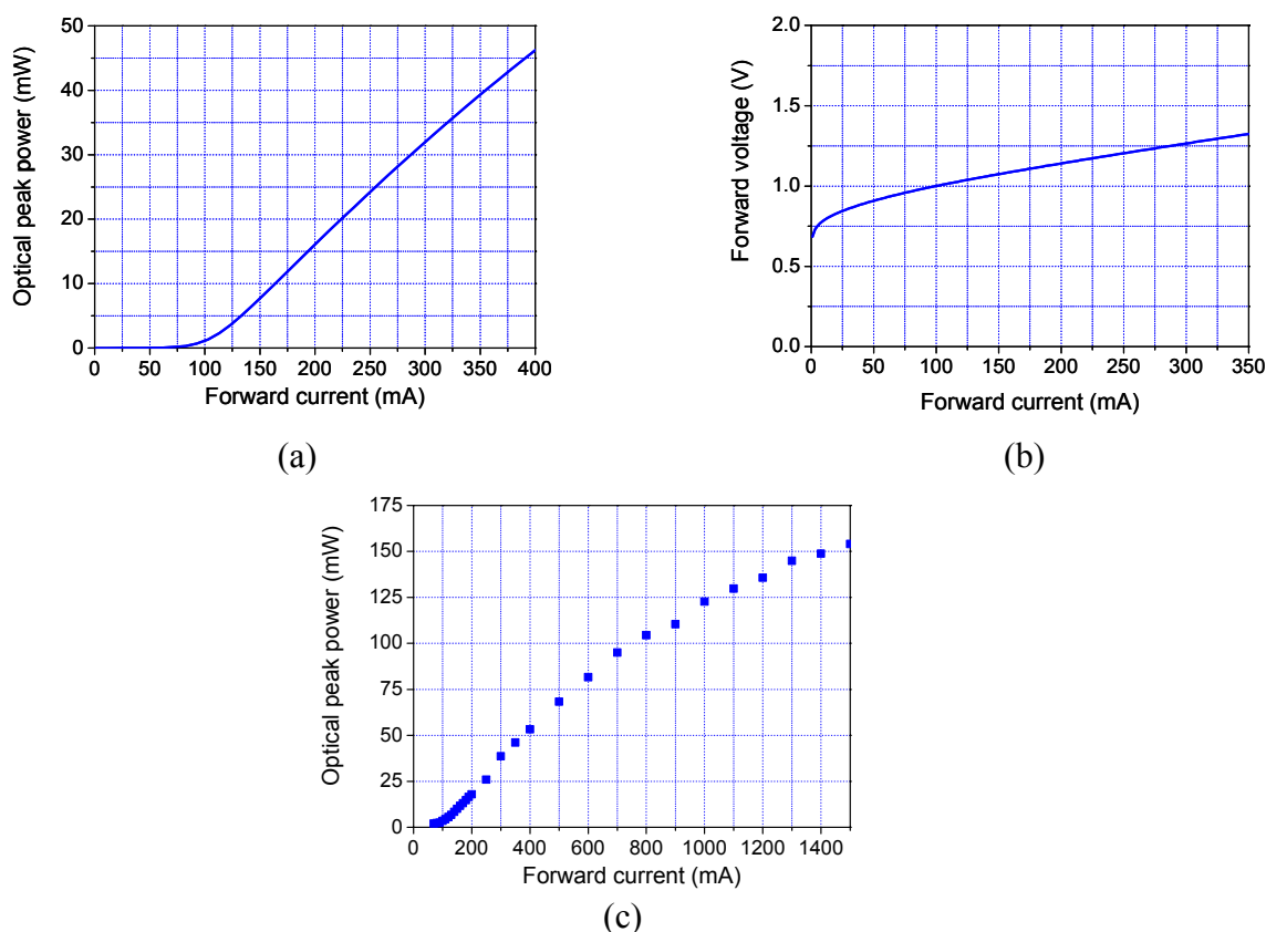
Figure 3.25: (a) CW power vs. forward current, (b) Forward voltage vs. forward current, and (c) Pulsed peak power vs. forward current with pulse width of 10ns, duty ratio of 0.1%
