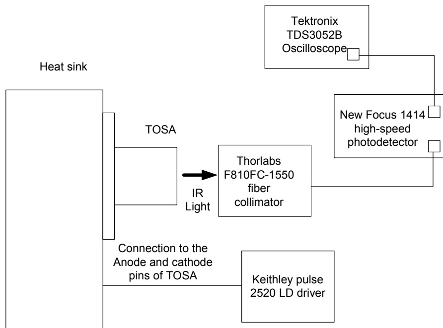
Figure 1b. Optical light source signal measurement setup
