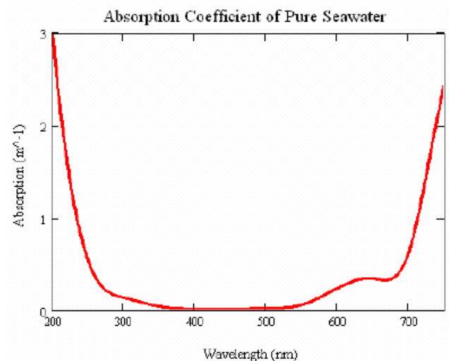
Figure 6-1: Spectral absorption coefficient of pure seawater 1
