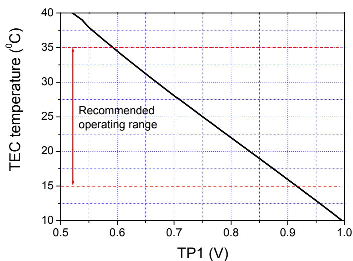
Figure 4-16: Dependence of TEC temperature with TP1 voltage
