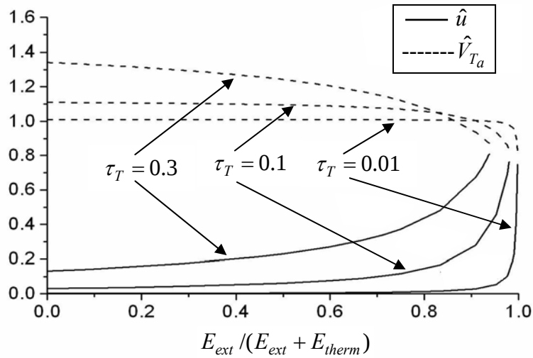
Figure 5. Parameters of the Knudsen layer as functions of ratio of external heat flux to the total heat flux at the ablating polyethylene surface
