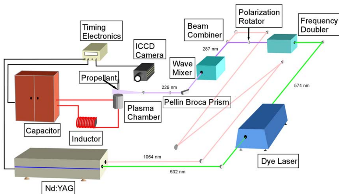
Figure A-2: NO PLIF laser setup.
