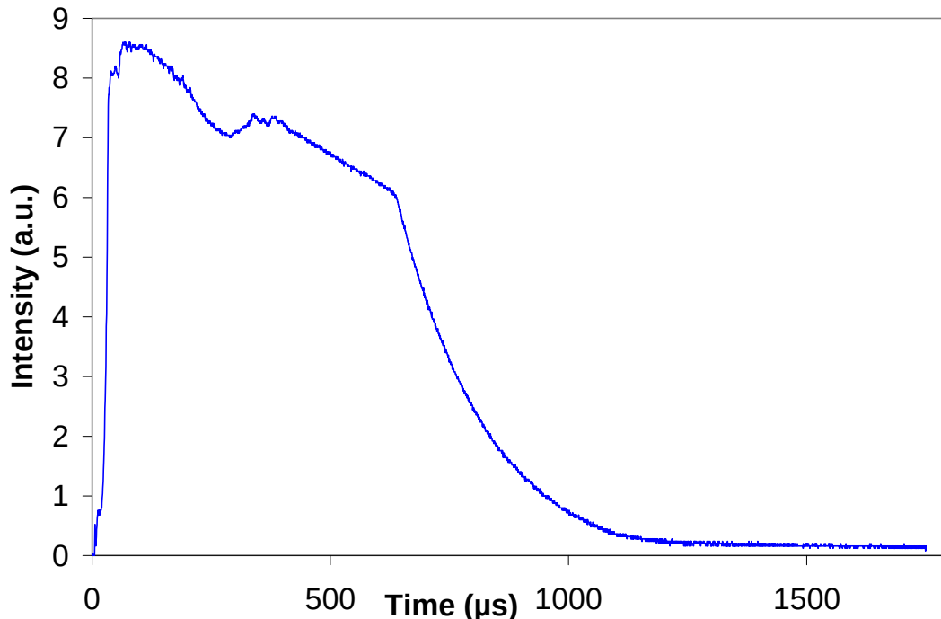
Figure 1: Plasma radiation intensity measured by a fast response photodiode
