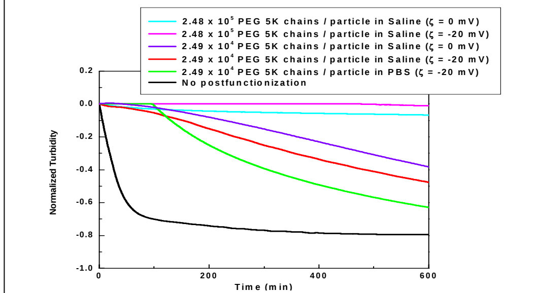
Figure 13: Plot of turbidity as a function of time. Turbidity used to assess stability of an aqueous solution of particles.
