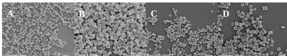
Figure 9 – SEM images of cylindrical PRINT particles (200 nm diameter \times 200 nm height) that have anti-mouse CD11b (A), anti-mouse CD11c (B), anti-mouse CD80 (C), and rat IgG2b (D) conjugated to the surface.
