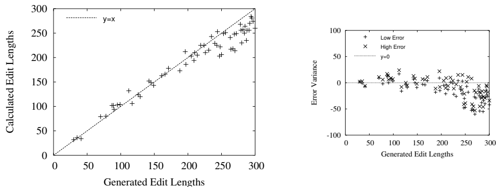
Fig. 4. Experimental results for 800 genes with expected edge length 40. Left: generated edit length vs. reconstructed length; right: the variance of computed distances per generated distance.
