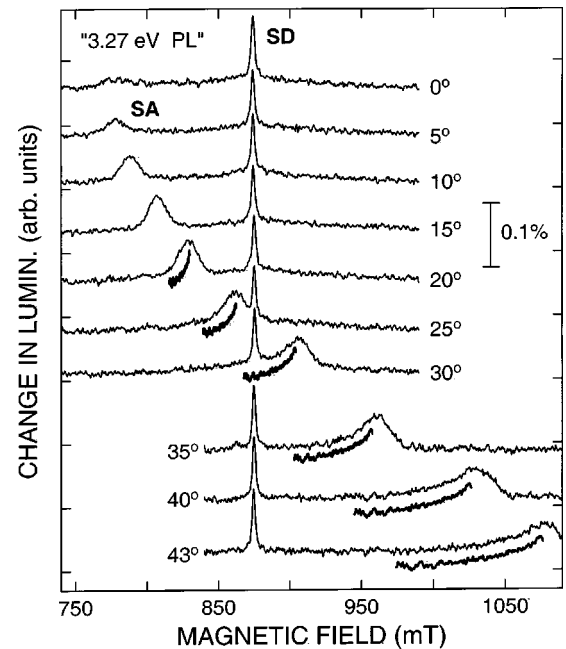
FIG. 2. ODMR spectra at 24 GHz detected on the 3.27-eV SD–SA PL for several orientations of the applied magnetic field ( \mathbf{B} ) in the (1120) plane ( 0^\circ refers to the c axis). The thick black curves (displaced vertically for clarity) are simulations of the low-field lineshapes for resonance SA as described in the text (SD, shallow donor; SA, shallow acceptor).
