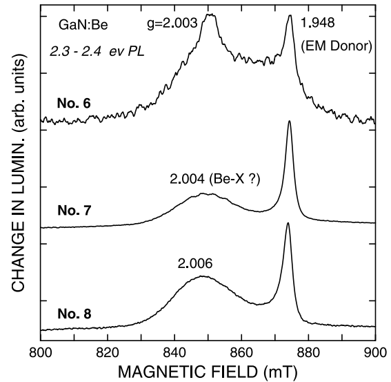
Fig. 10. ODMR found on the 2.3 – 2.4 eV PL bands from Be-doped GaN with \mathbf{B} \perp c . The broad feature with g = 2.004 \pm 0.002 is likely associated with a Be-related (deep) acceptor complex as suggested in [49].
