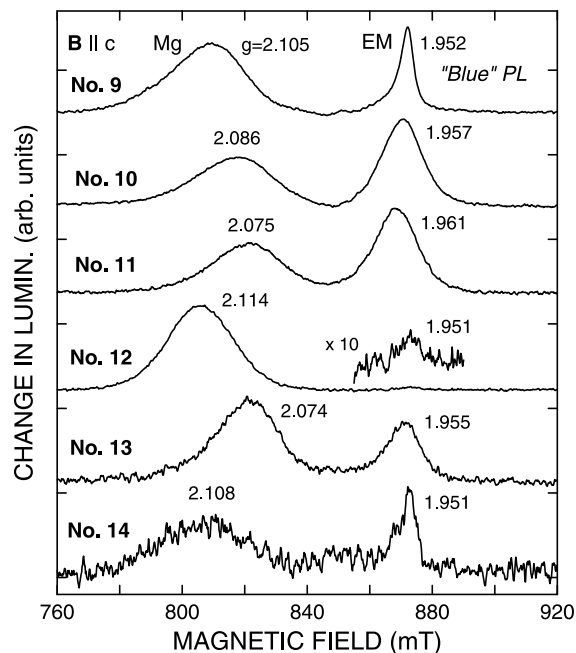
Fig. 8. ODMR found on the ‘blue’ emission bands from six Mg-doped GaN layers with \mathbf{B} \parallel c . The feature with g \sim 2.1 is attributed to Mg shallow acceptors.
