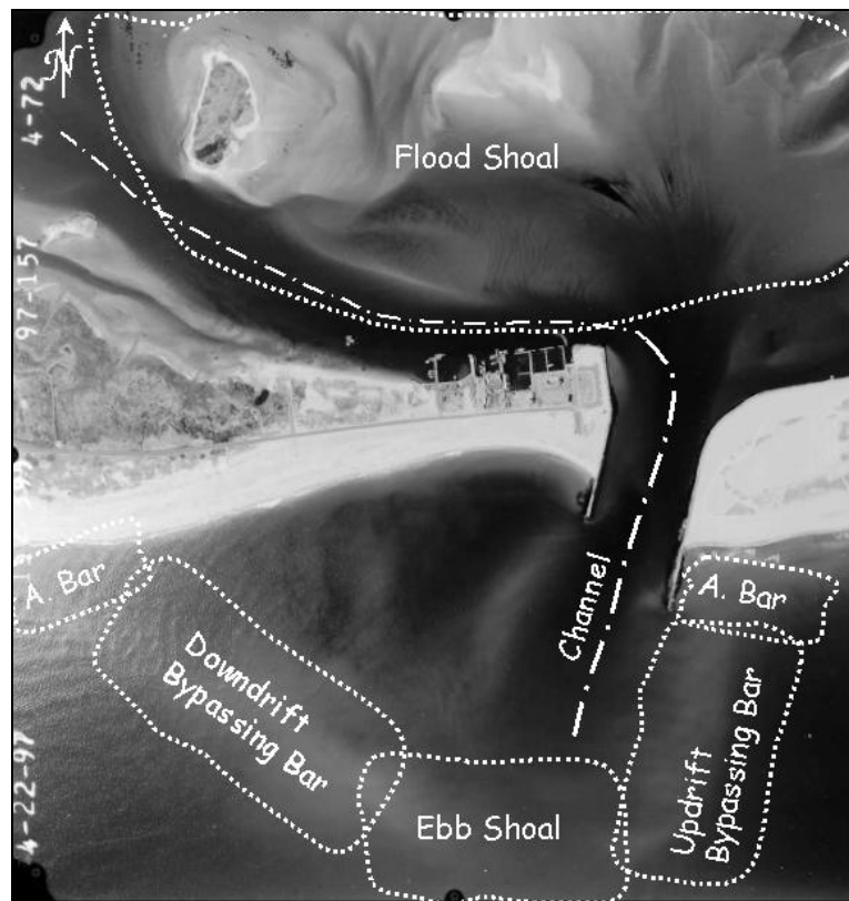
Fig. 1. Morphologic features, Shinnecock Inlet, New York
