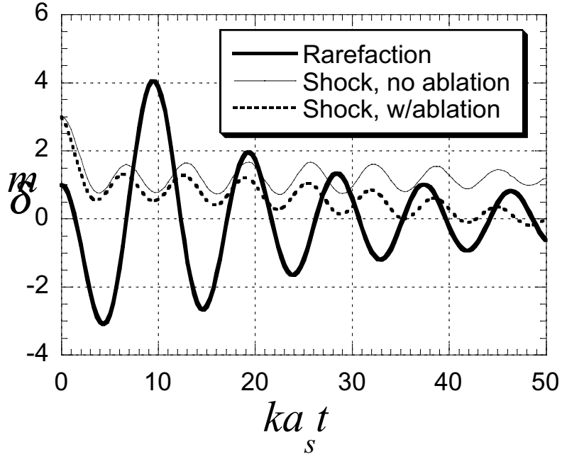
Fig. 1. Time history of normalized mass variation in a planar target caused by a rippled rarefaction wave and a rippled shock wave (small-amplitude theory). Initial amplitudes of the front and rear surface ripples are the same; the time origin for the rarefaction curve is shifted to the shock breakout at the rippled rear surface.
