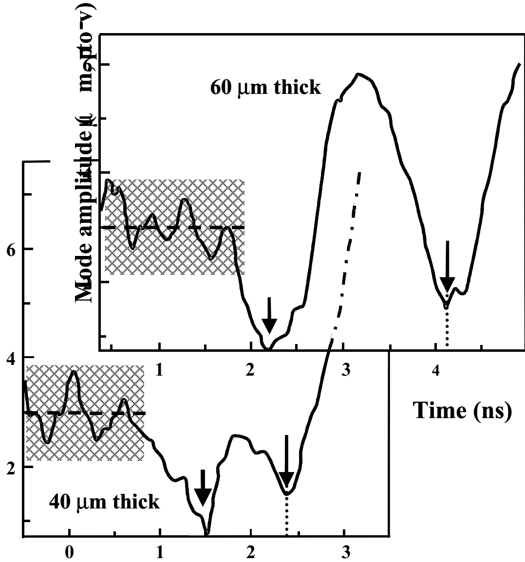
Fig. 3. Peak-to-valley amplitudes of the dominant Fourier modes for 40 μm and 60 μm thick targets vs. time. 2a_0 = 3 \mu\text{m} , \lambda = 45 \mu\text{m} , peak laser intensity 5 \times 10^{13} \text{ W/cm}^2 . First and second phase reversals are marked on both pictures. The thickness of the shaded area corresponds to the experimental uncertainty of the mode amplitude measurement.
