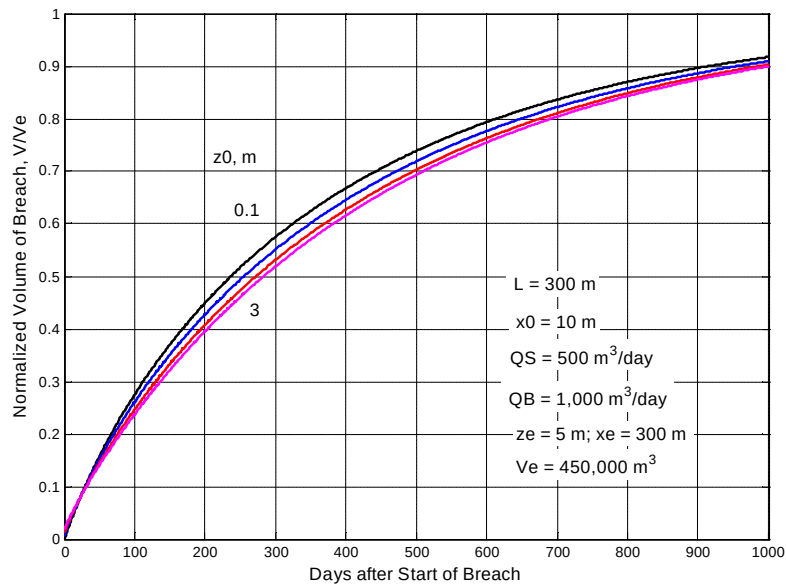
Fig. 7. Growth of breach volume for fixed initial width and different initial depths corresponding to Figs. 5 and 6.
