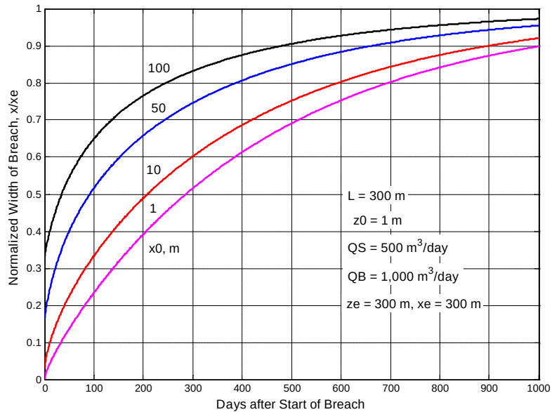
Fig. 8. Solution of Eq. (4) for breach width, different values of initial breach width.
