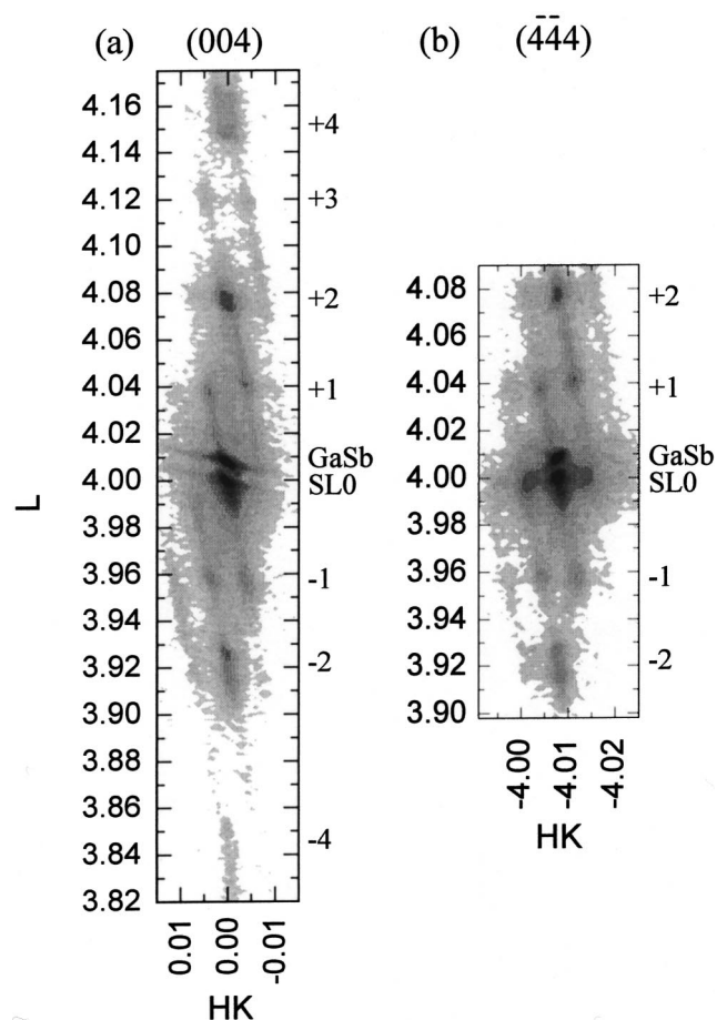
FIG. 5. XRD reciprocal space maps of LCM around the (a) (004) and (b) (444) Bragg peaks at \phi=90^\circ , parallel to the LCM, whose linear radial scan is shown in Fig. 3(b).
