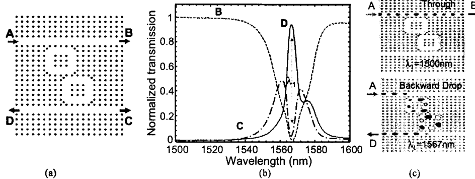
Fig. 6. Dual-ring PCRR ADF for backward-dropping: (a) Schematic showing the weakly coupled dual PCRR rings with coupling period of 2a ; (b) Normalized transmission spectra; (c) The field patterns of electric field distribution for "through" (off-resonance: \lambda_0 = 1500 nm) and "backward drop" (on-resonance: \lambda_1 = 1567 nm) channels.
