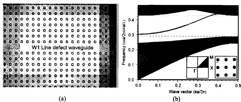
Fig. 3. (a) Single line-defect (W1) photonic crystal waveguide; (b) Dispersion plot and the corresponding defect mode shown as a blue line in the photonic bandgap region.
