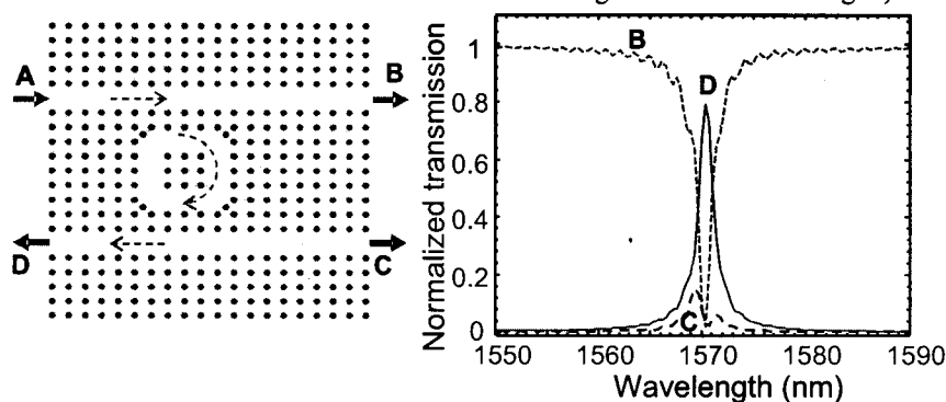
Fig. 5. Single-ring PCRR based ADF with higher spectral selectivity ( Q > 1000 , \delta\lambda = 1.5\text{nm} at \lambda_1 = 1571\text{nm} ), by increasing the coupling periods between W1 waveguide and PCRR cavity from one to two.
