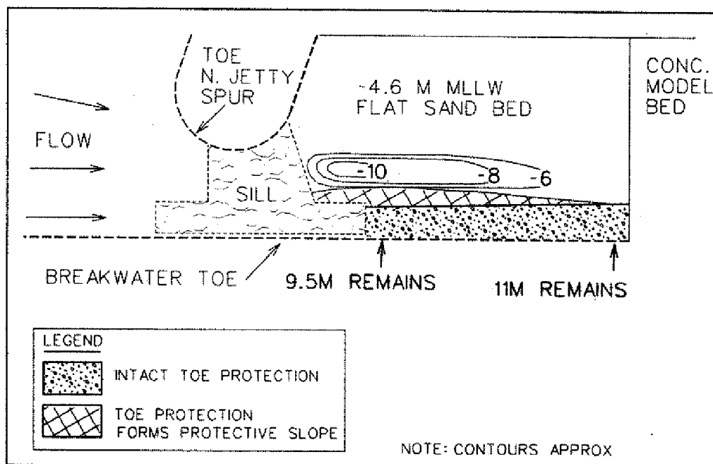
Figure 6: Plan 3 detached breakwater toe protection.
