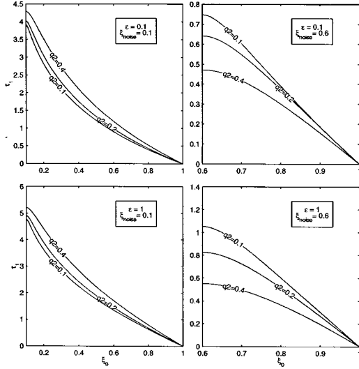
Figures 6. Dependence of \tau_1(\bar{\xi}_0, \bar{\xi}_{noise}, q^2) on the initial condition error \bar{\xi}_0 for three different values of the stochastic forcing q^2 (0.1, 0.2, and 0.4) using Nicolis model with Two different values of \epsilon (0.1, and 1) and two different values of noise level \bar{\xi}_{noise} (0.1, and 0.6).
