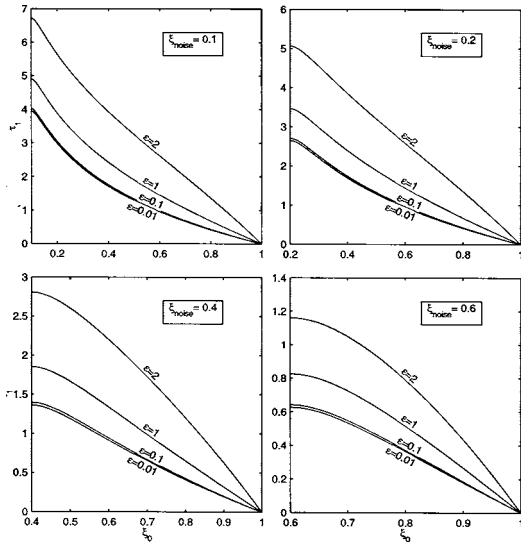
Figures 4. Dependence of \tau_1(\bar{\xi}_0, \bar{\xi}_{noise}, \varepsilon) on the initial condition error \bar{\xi}_0 for four different values of \varepsilon (0.01, 0.1, 1, and 2) and four
