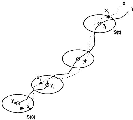
Figure 1. Phase space trajectories of model prediction y (solid curve) and reality x (dashed curve) and error ellipsoid S_d(t) centered at y . The positions of reality and prediction trajectories at time instance are
