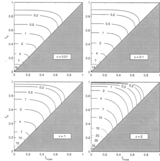
Figures 3. Contour plots of \tau_2(\bar{\xi}_0, \bar{\xi}_{noise}, \varepsilon) versus (\bar{\xi}_0, \bar{\xi}_{noise}) for four different values of \varepsilon (0.01, 0.1, 1, and 2) using Nicolis model with stochastic forcing q^2 = 0.2 . The contour plot covers the half domain due to \bar{\xi}_0 \geq \bar{\xi}_{noise} .
