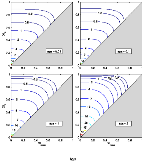
Figures 3. Contour plots of \tau_2(\bar{\xi}_0, \bar{\xi}_{noise}, \epsilon) versus (\bar{\xi}_0, \bar{\xi}_{noise}) for four different values of \epsilon (0.01, 0.1, 1, and 2) using Nicolis model with stochastic forcing.
