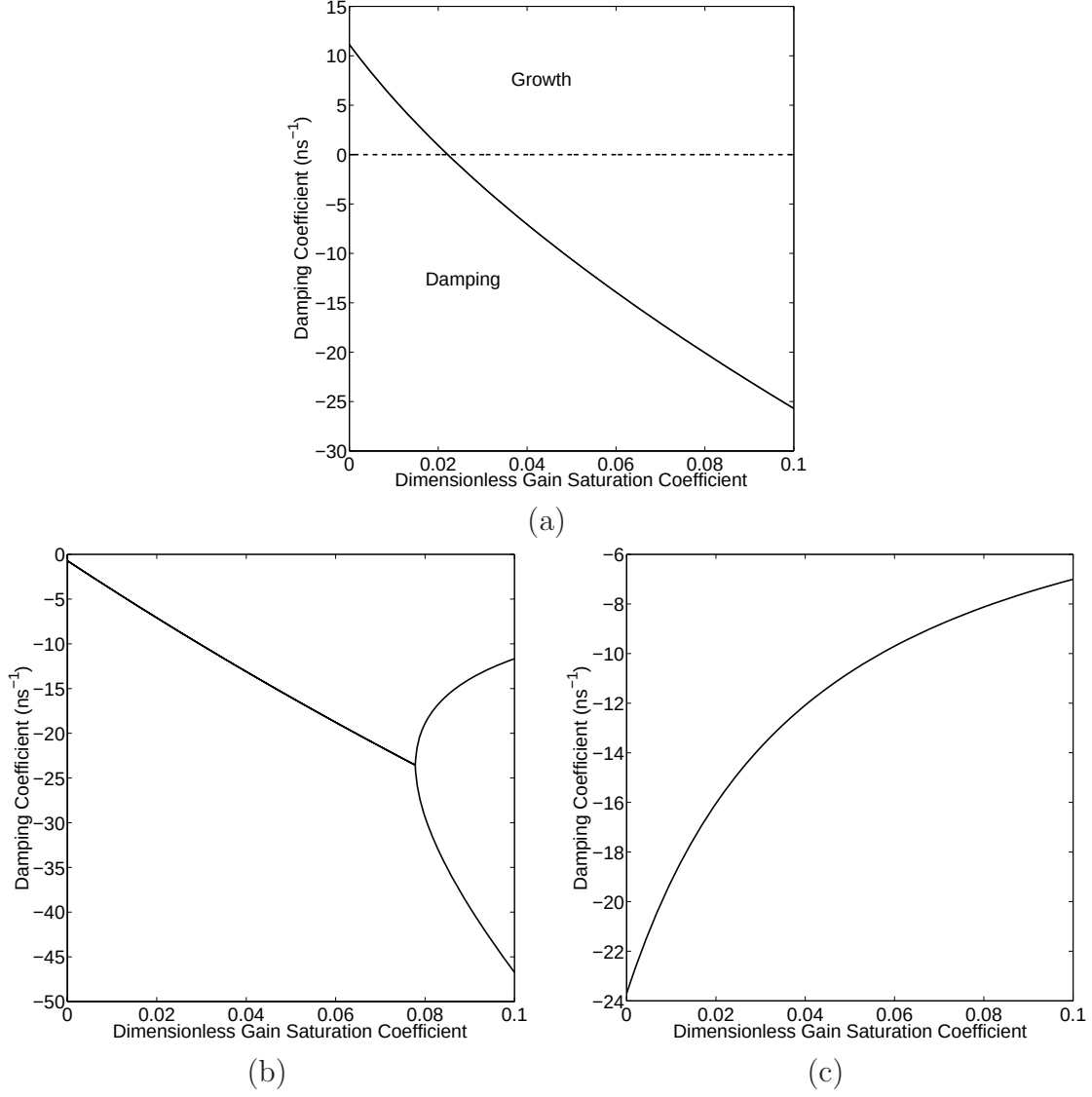
Figure 12. Damping coefficients vs. dimensionless gain saturation coefficient. The steady states become stable at a coefficient value of about 0.02 where the coefficient in (a) becomes negative. The split in (b) is due to the associated resonance frequency becoming imaginary.
