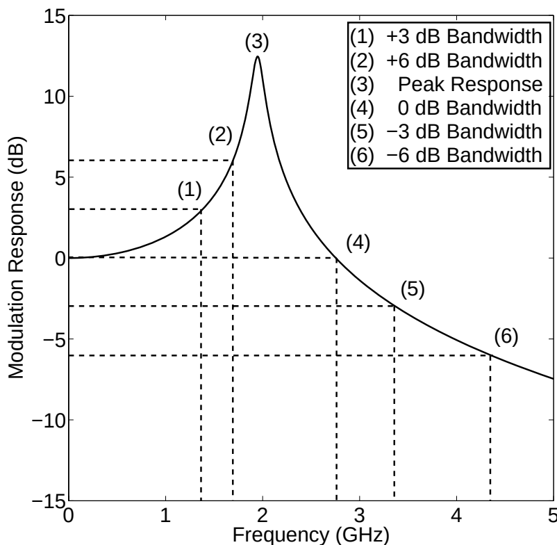
Figure 1. Some properties of the modulation response for a solitary InGaAsP diode laser. Adapted from Reference [1] and Reference [14].
