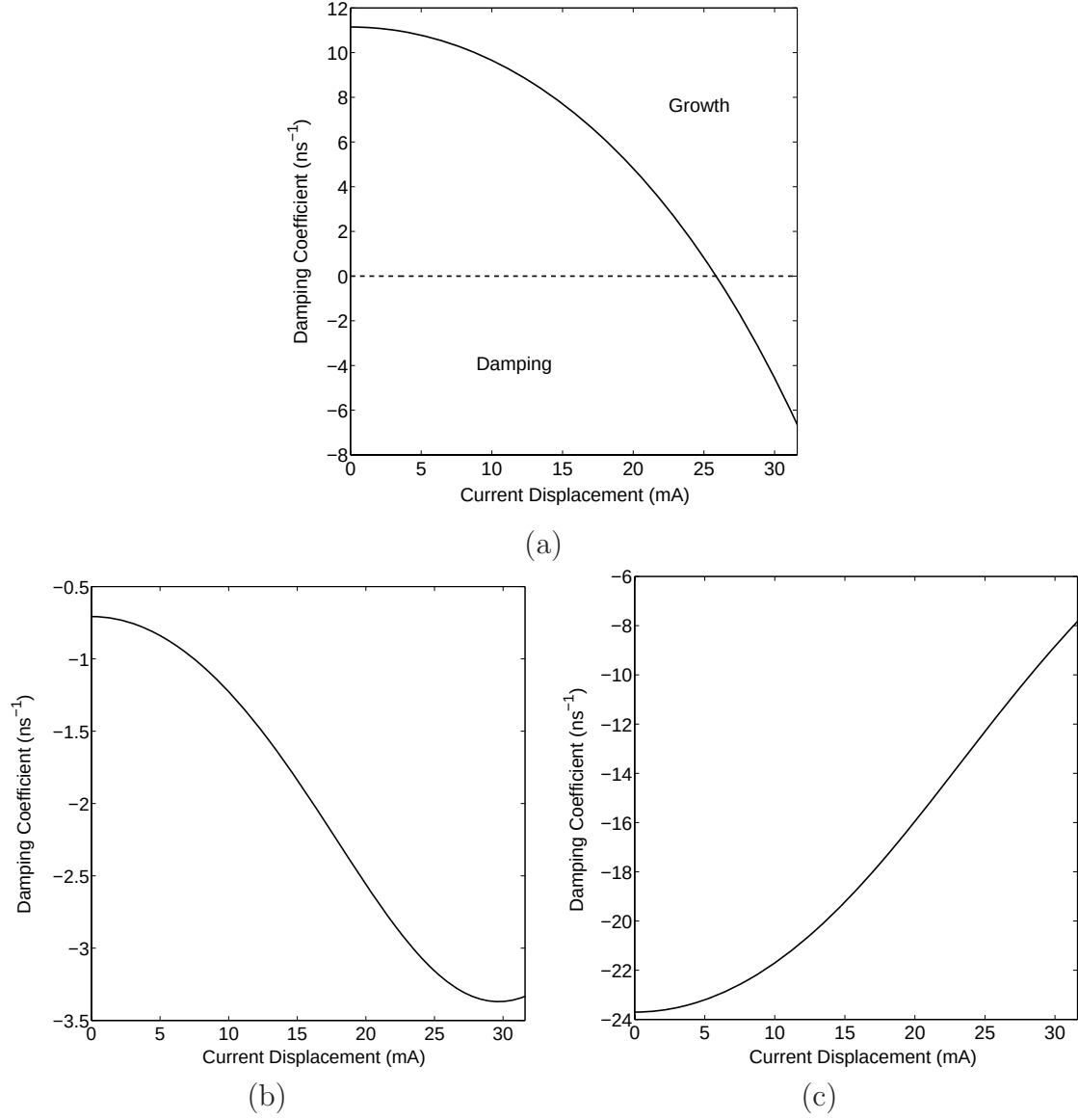
Figure 9. Damping coefficients vs. current displacement. The steady states become stable at about 25 mA of current displacement where the coefficient in (a) becomes negative.
