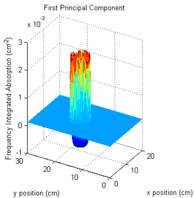
Figure 26.b. The first principal component for the 1216 cm -1 transition
