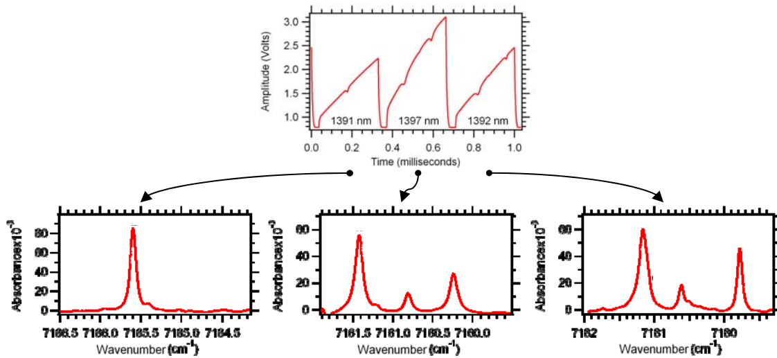
Figure 14. A single period of the raw data from the three multiplexed lasers with the corresponding absorption spectra
