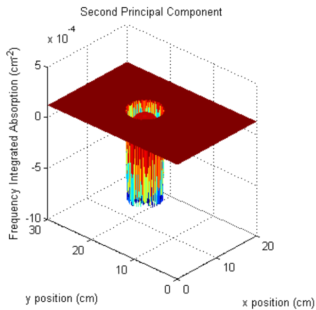
Figure 26.c. The second principal component for the 1216 cm -1 transition
