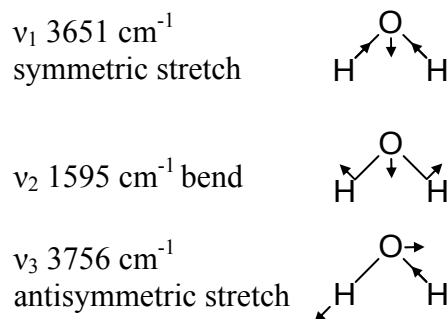
Figure 1. The normal modes of vibration of \text{H}_2\text{O}
