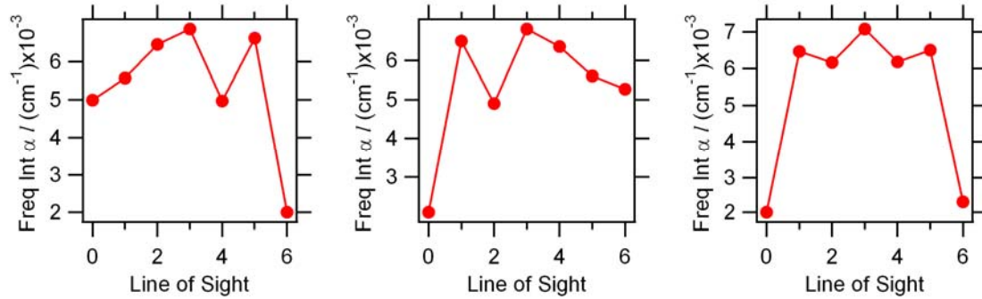
Figure 16. Integrated absorption of the 1216 cm -1 transition for each of the seven lines of sight with the flame 9 mm left of center, in the center position, and 9 mm right of center
