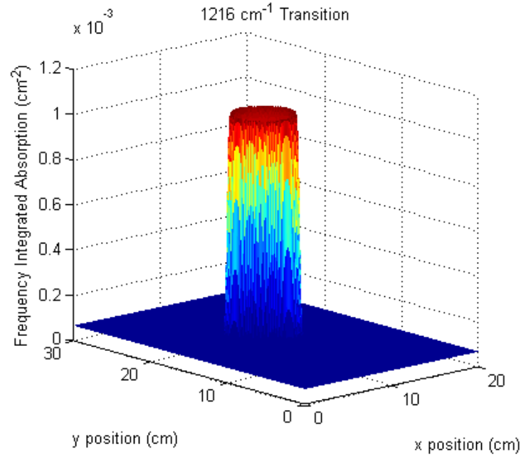
Figure 27.c. Fit absorption map for the 1216 cm -1 transition
