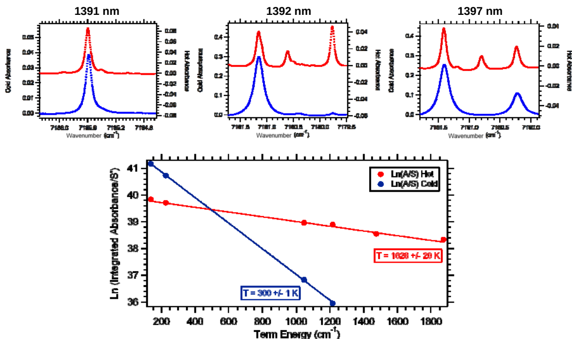
Figure 19. Separated spectra and Boltzmann plots resulting from peak integrations
