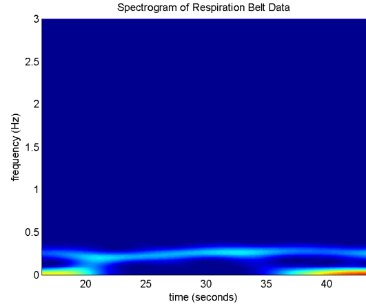
(d) The spectrogram of (c), showing a respiration rate of about 0.25 Hz, meaning the subject takes approximately 1 breath every 4 seconds. This breath rate may be determined from the radar data.
