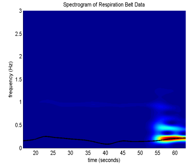
(f) The breath rate estimate on top of the spectrogram of the respiration belt signal.
