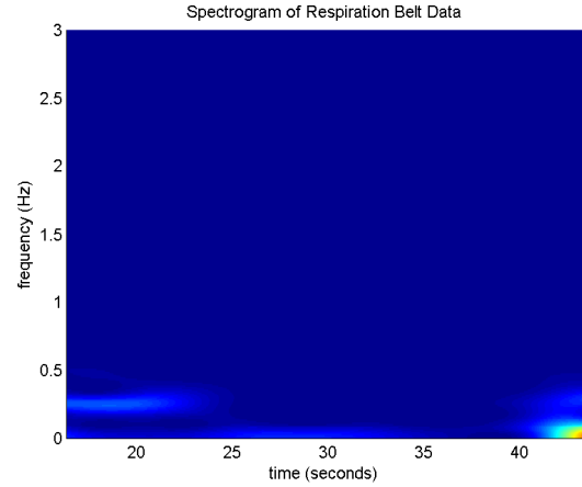
(d) The spectrogram of (c) showing that the subject is holding his breath between 25 and 40 seconds. During the first 25 seconds, the subject is breathing, and we can see that the subject's breath rate is about 0.25 Hz, meaning the subject takes approximately 1 breath every 4 seconds. This breath rate may be determined from the radar data.
