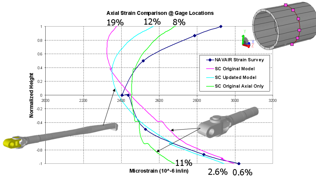
Figure 58: Comparison of predicted axial strains and strain survey results (axial load of 137 kip).
