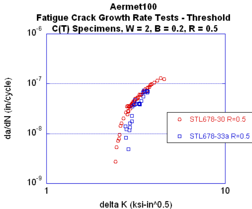
Figure 3.4.3-9. FCGR threshold data at R= 0.5.
