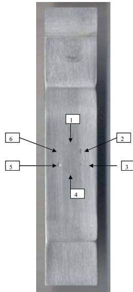
Figure 3.2.1-2. Typical micro-machined specimen.
