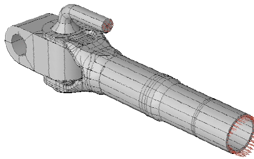
Figure 17: Arrestment hook local 3D-model for the damper load case
