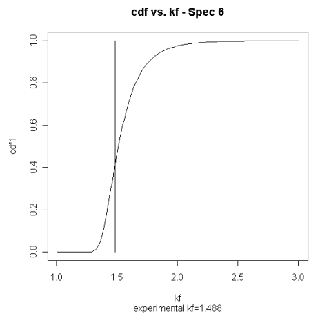
Figure 4.1-3. Calibrated ESR model prediction and plate critical k_f for AF1410 Set A Specimen 6.
