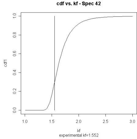
Figure 4.1-1. Calibrated ESR model prediction and plate critical k_f for AF1410 Set A Specimen 42.
