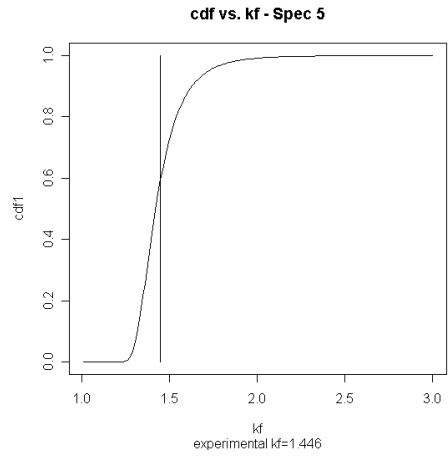
Figure 4.1-2. Calibrated ESR model prediction and plate critical k_f for AF1410 Set A Specimen 5.
