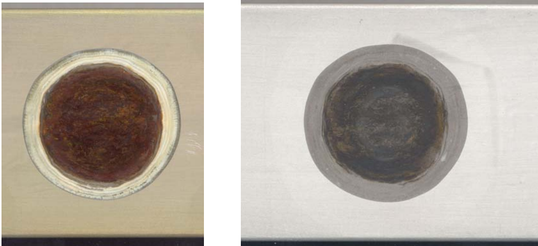
Figure 3.3.3-4. Cadmium-plated corrosion-fatigue test, Specimen 614-14 pre- and post-cleaning.
