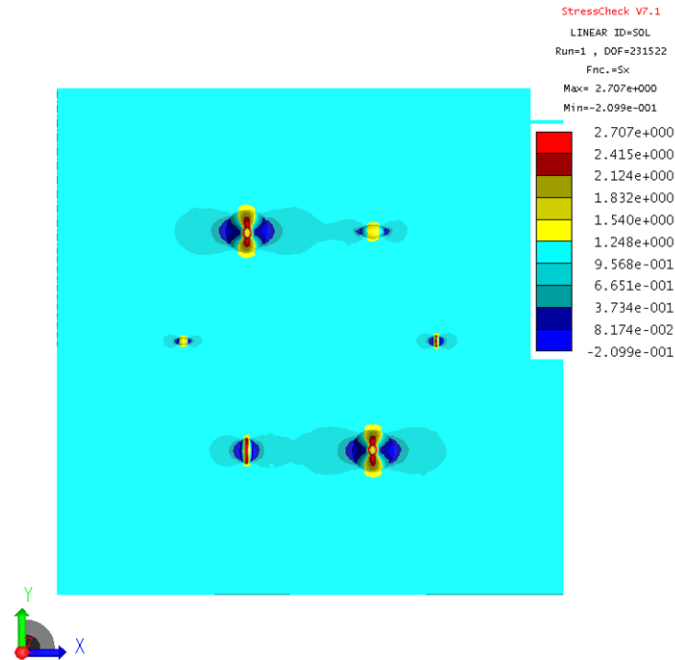
Figure 72: Fringe Plot of Kt for WLI-Measured Dimensions
