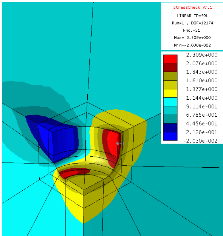
Figure 67: Kt-value for R=0.375
