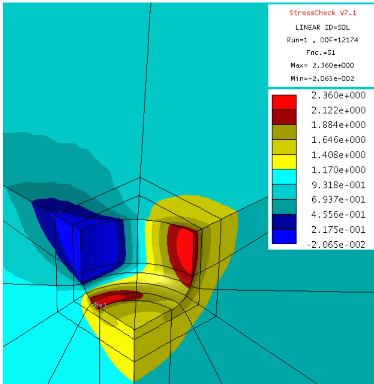
Figure 66: Kt-value for R=0.35
