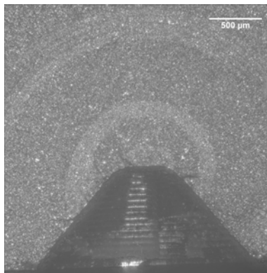
Figure 3.2.1-4. Deep-focus image of Specimen 598-7 – Crack 1 at Feature #2.
