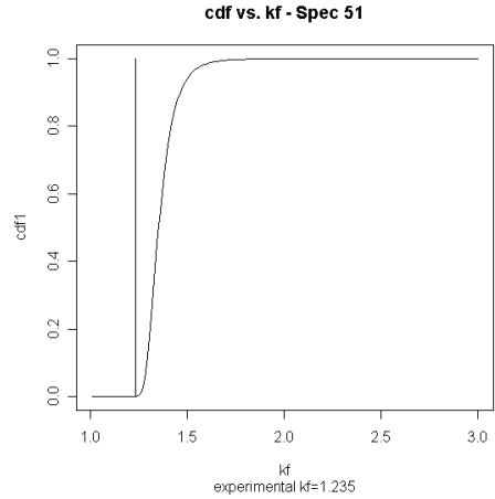
Figure 4.1-4. Calibrated ESR model prediction and plate critical k_f for AF1410 Set A Specimen 51.
