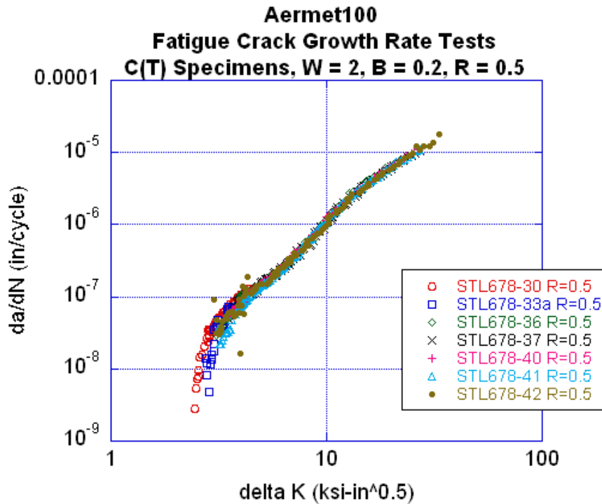
Figure 3.4.3-4. FCGR data at R = 0.5 with threshold.
