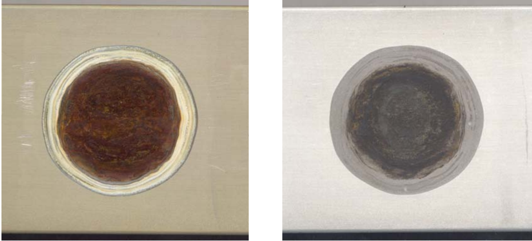
Figure 3.3.3-3. Cadmium-plated corrosion-fatigue test, Specimen 614-10 pre- and post-cleaning.
