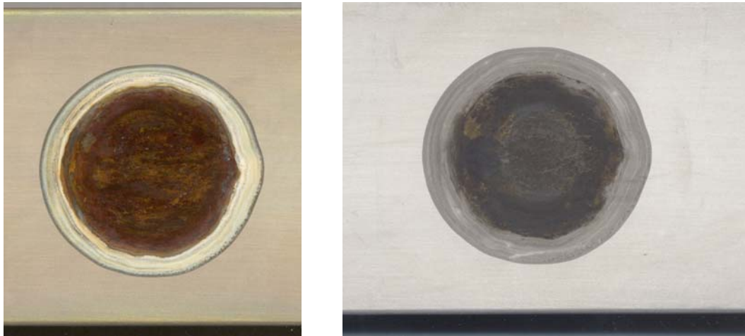
Figure 3.3.3-5. Cadmium-plated corrosion-fatigue test, Specimen 614-23 pre- and post-cleaning.
