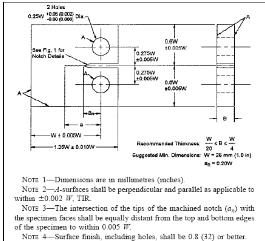
Figure 3.4.3-1. C(T) specimen.
