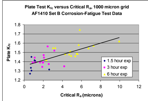
Figure 4.2-2. Plate test k_{fc} versus critical R_a for a 1000-micron grid for AF1410 Set B corrosion-fatigue test data.
