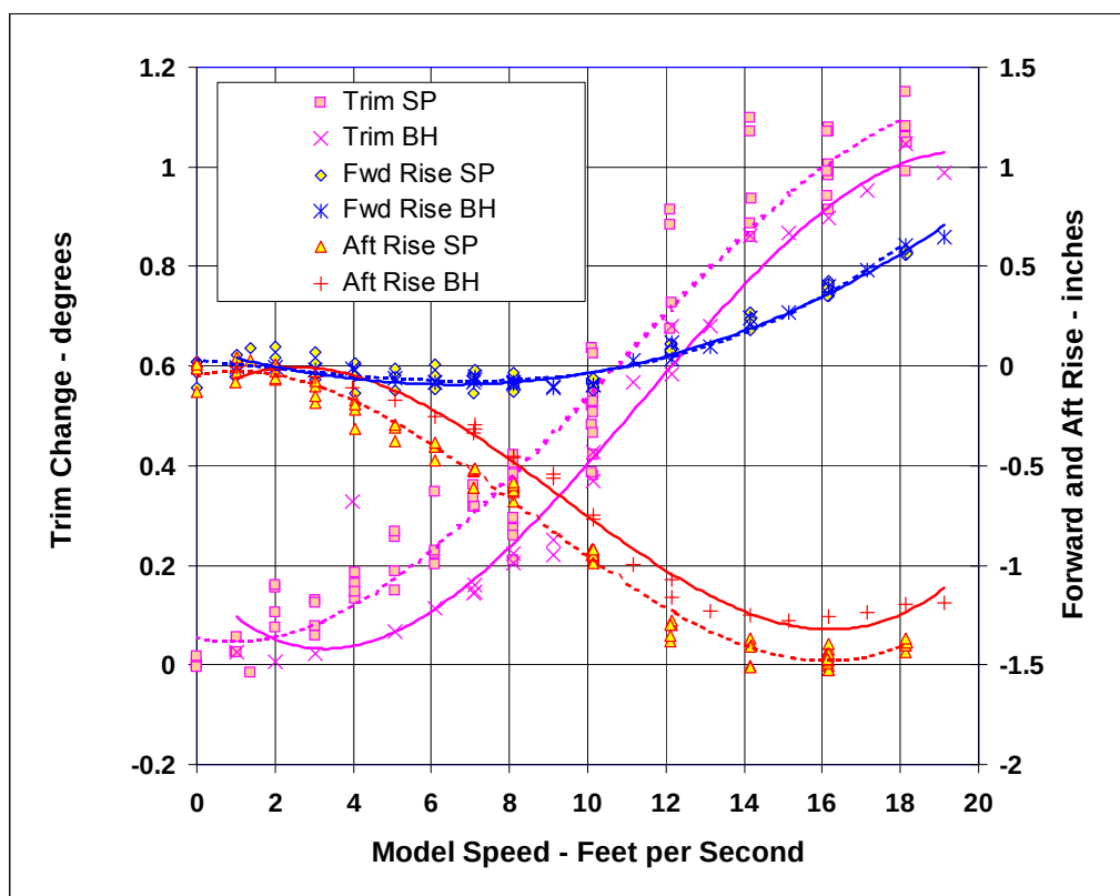
FIGURE 5. COMPARISON OF BARE HULL AND SELF-PROPULSION TRIM AND FORE AND AFT RISE
